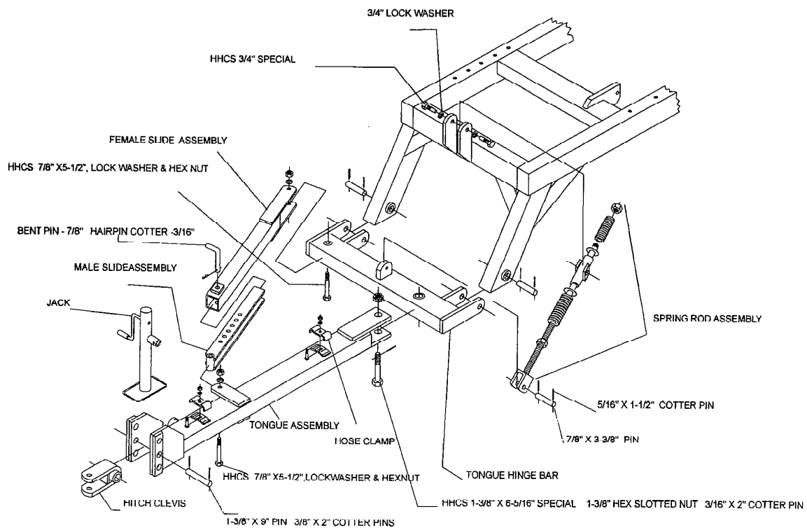
Figure 5 - Tongue & Spring Rod Assembly
