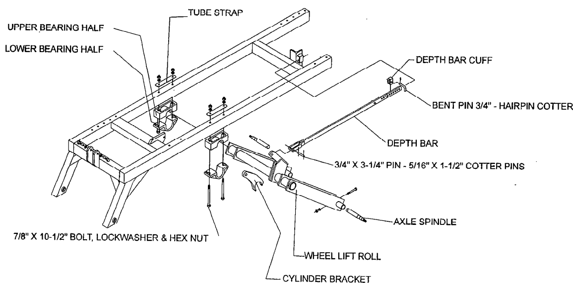
Figure 6 - Wheel Lift Assembly
