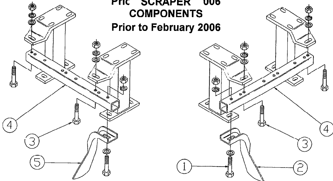
FIGURE 11 SCRAPER COMPONENTS
