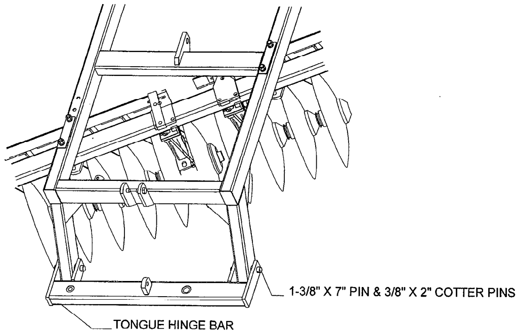
Figure 4 - Hitch Assembly
